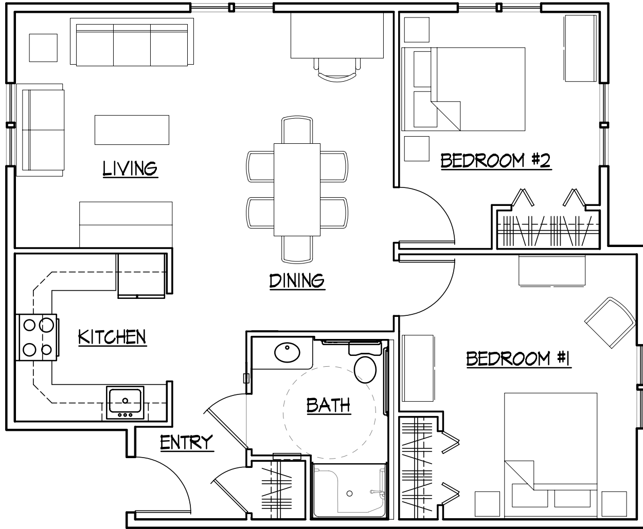
2 P5 TWO BEDROOM TYPE "B" 1/4"=1'-0" (3 UNITS) 860 SF.
