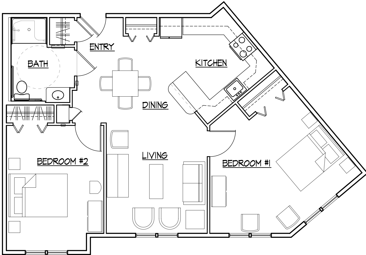
3 TWO BEDROOM TYPE "C" P5 1/4"=1'-0" (3 UNITS) 885 S.F.
