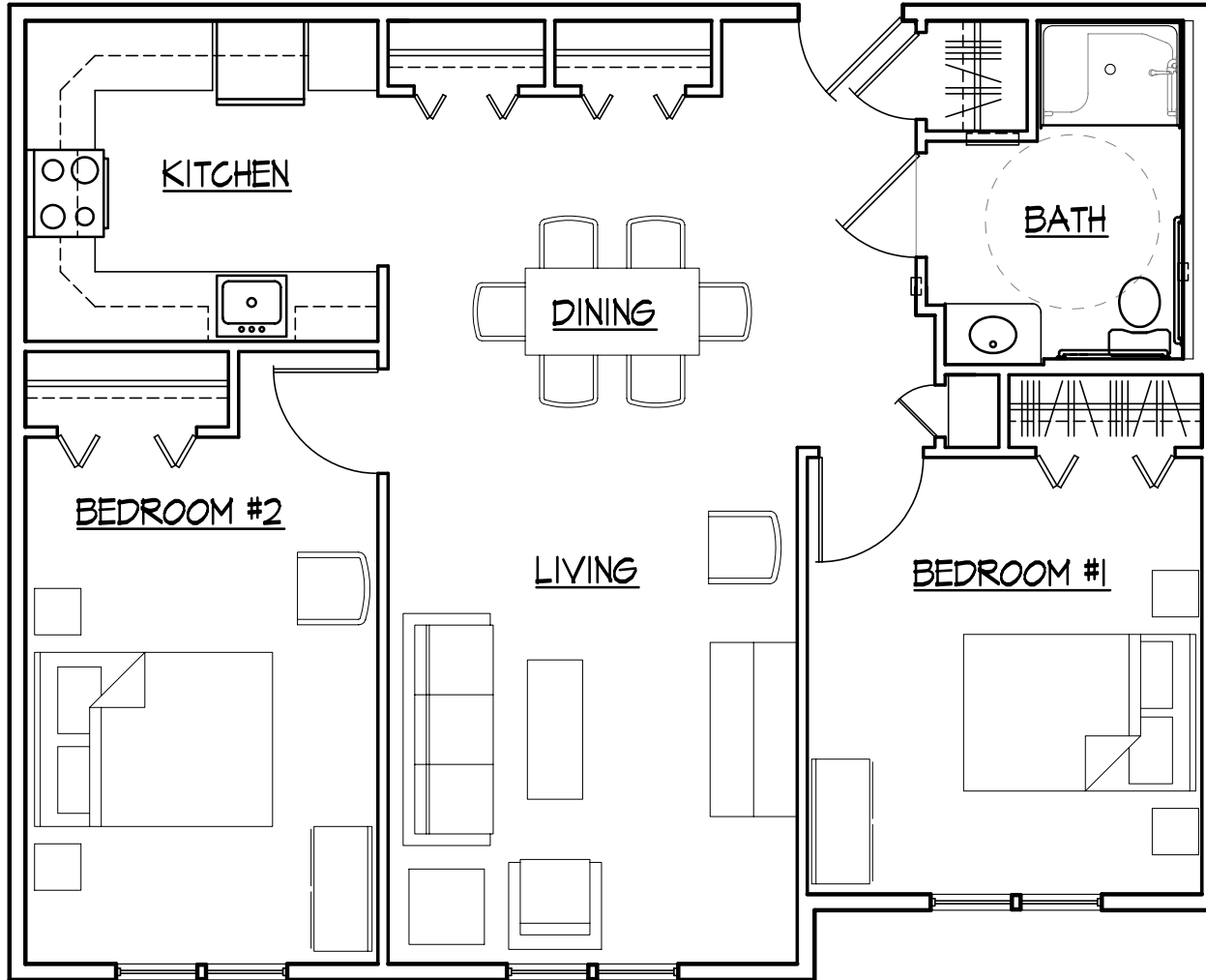
4 P5 TWO BEDROOM TYPE "D" 1/4"=1'-0" (3 UNITS) 885 SF.
